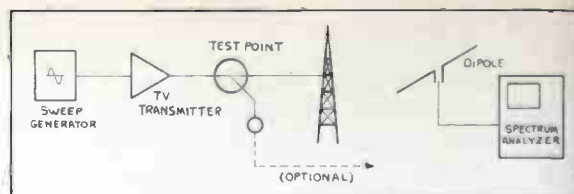
Fig. 12 Set-up procedure No. 4. Equipment required: 7L12 or 7L13 Spectrum Analyzer; 7613 variable persistence or 7313 storage mainframe; Wavetek 1801A38 sweep generator with 15 KHz modulator.
