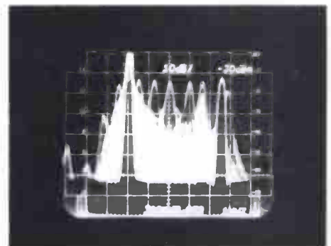
Fig. 11 In-service VIT sideband analysis using multiburst.
